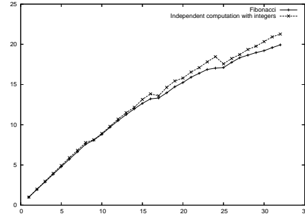
Figure 11: Fibonacci with granularity control vs. maximum speedup in a real machine.
