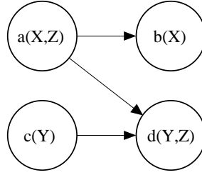
Figure 2: Dependency graph for p/3 .
