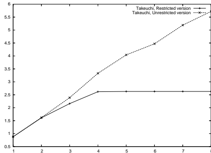
Figure 10: Restricted and unrestricted IAP versions of Takeuchi .
