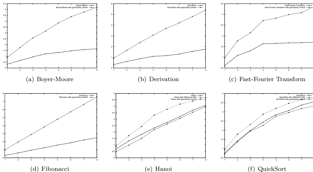
Figure 9: Speedups for some selected benchmarks with and without granularity control.
