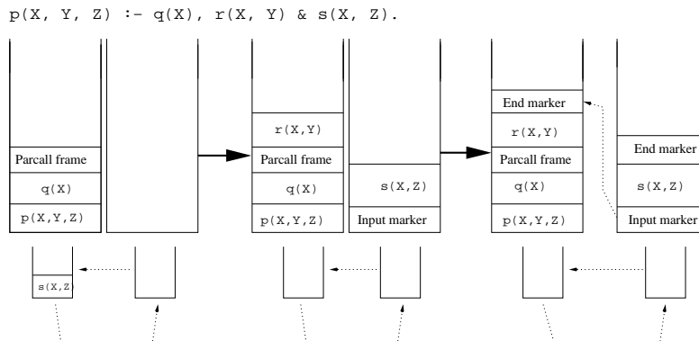
Figure 1: Sketch of data structures layout using the marker model.
