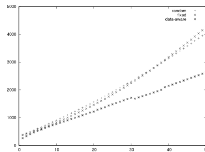
Figure 16: Two-tier simulation results for p_f = 0.8 .
